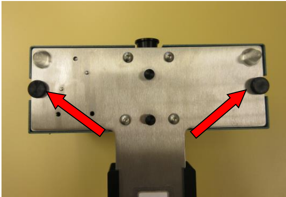
Figure 5.1.1 Cover screws
